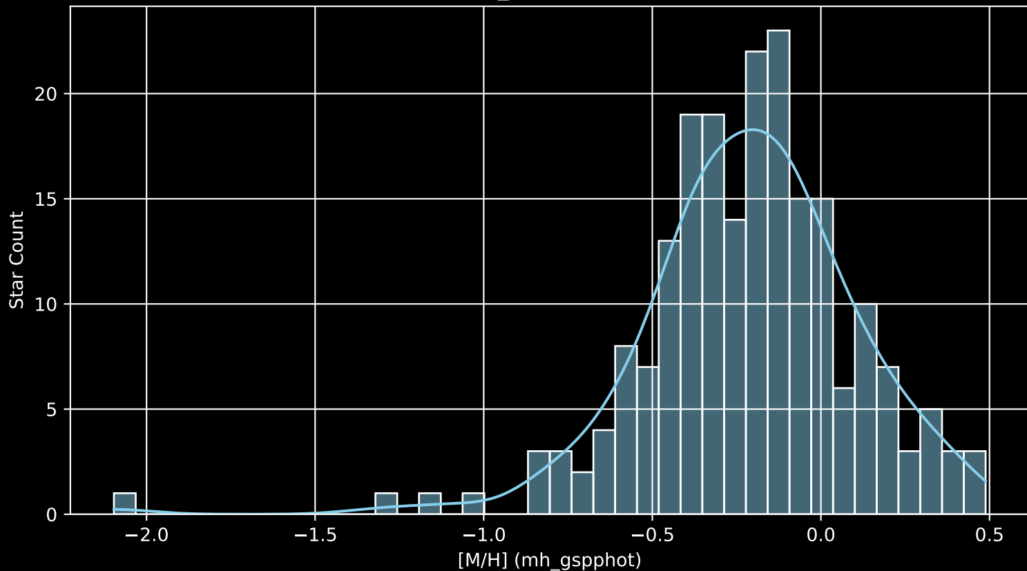
APOGEE DR17 Field: [CVZ_OB01_btx [M/H] (mh_gspphot) (n= 208)
