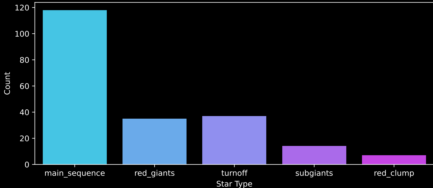
APOGEE DR17 Field: [CVZ_OB01_btx] Count plot of Star Type
