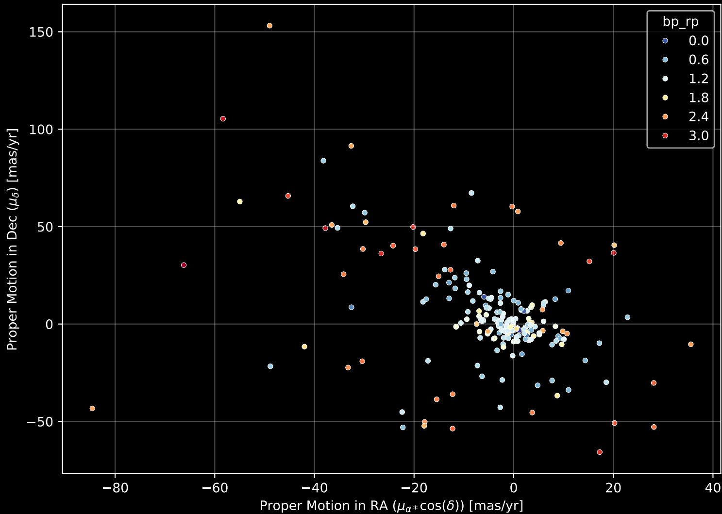
APOGEE DR17 Field: [CVZ_OB01_btx] Proper Motion Diagram (n= 211)
