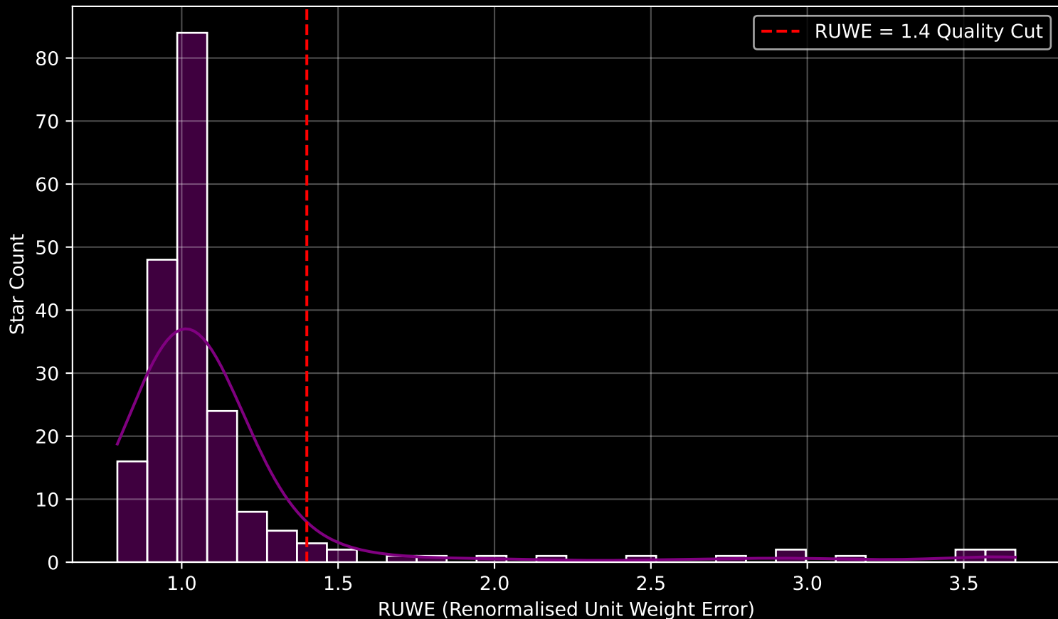
GAPOGEE DR17 Field [CVZ_OB01_btx] RUWE Distribution (n= 203)
