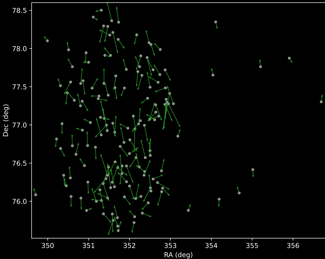
APOGEE DR17 Cluster 4 Proper Motion Vectors (n=150)
