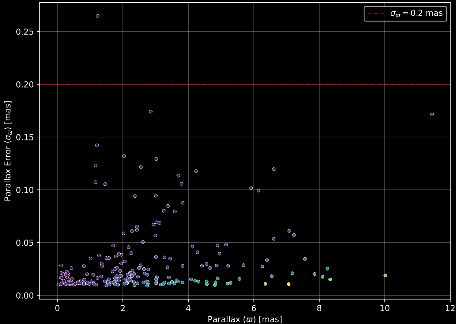
APOGEE DR17 Field: [CVZ_OB01_btx] Parallax Quality (n= 211)
